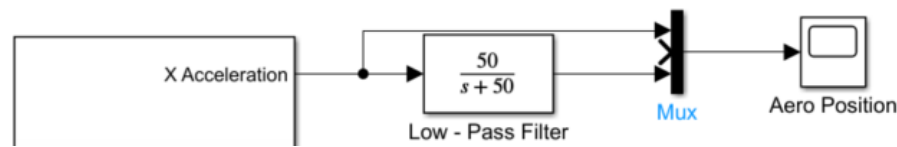
Figure 2: X-axis acceleration signal with a low-pass filter
