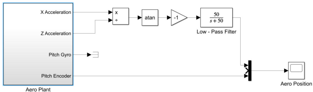
Figure 3: Calculating angle from acceleration
