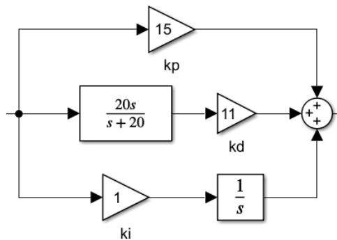
Figure 5: PID gains in a feedback loop
