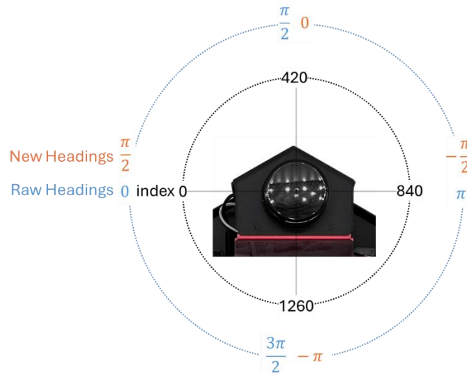
Figure 3. LiDAR measurement correction
