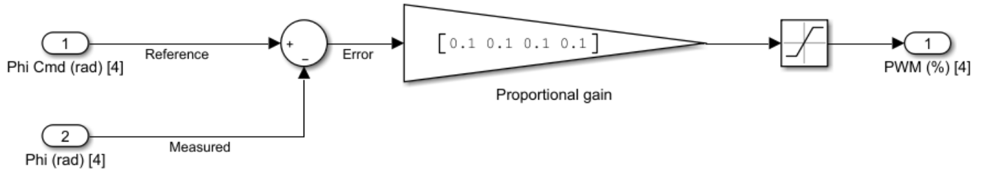
Figure 2.2 Proportional Controller
