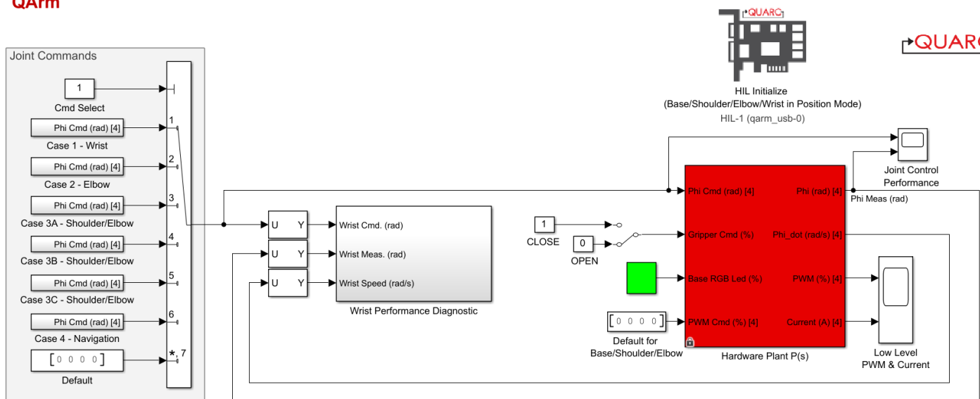
Figure 13: Simulink model for QArm in position mode
