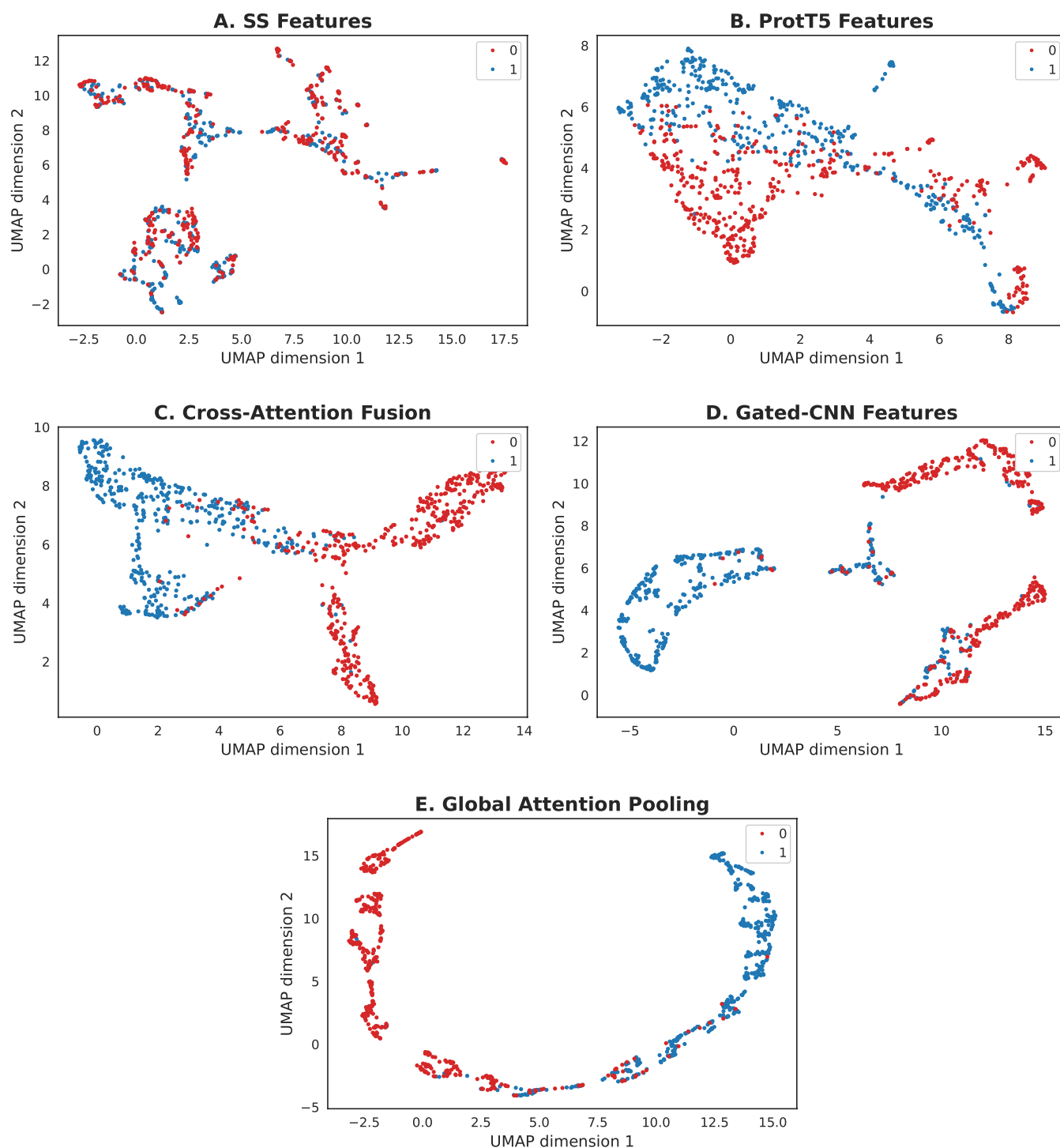
Figure 4. Feature visualizations on the independent test set. (A) SS8 features. (B) ProtT5 embeddings. (C) Gated cross-attention features. (D) Multiscale gated convolution features. (E) Global attention pooling features.
