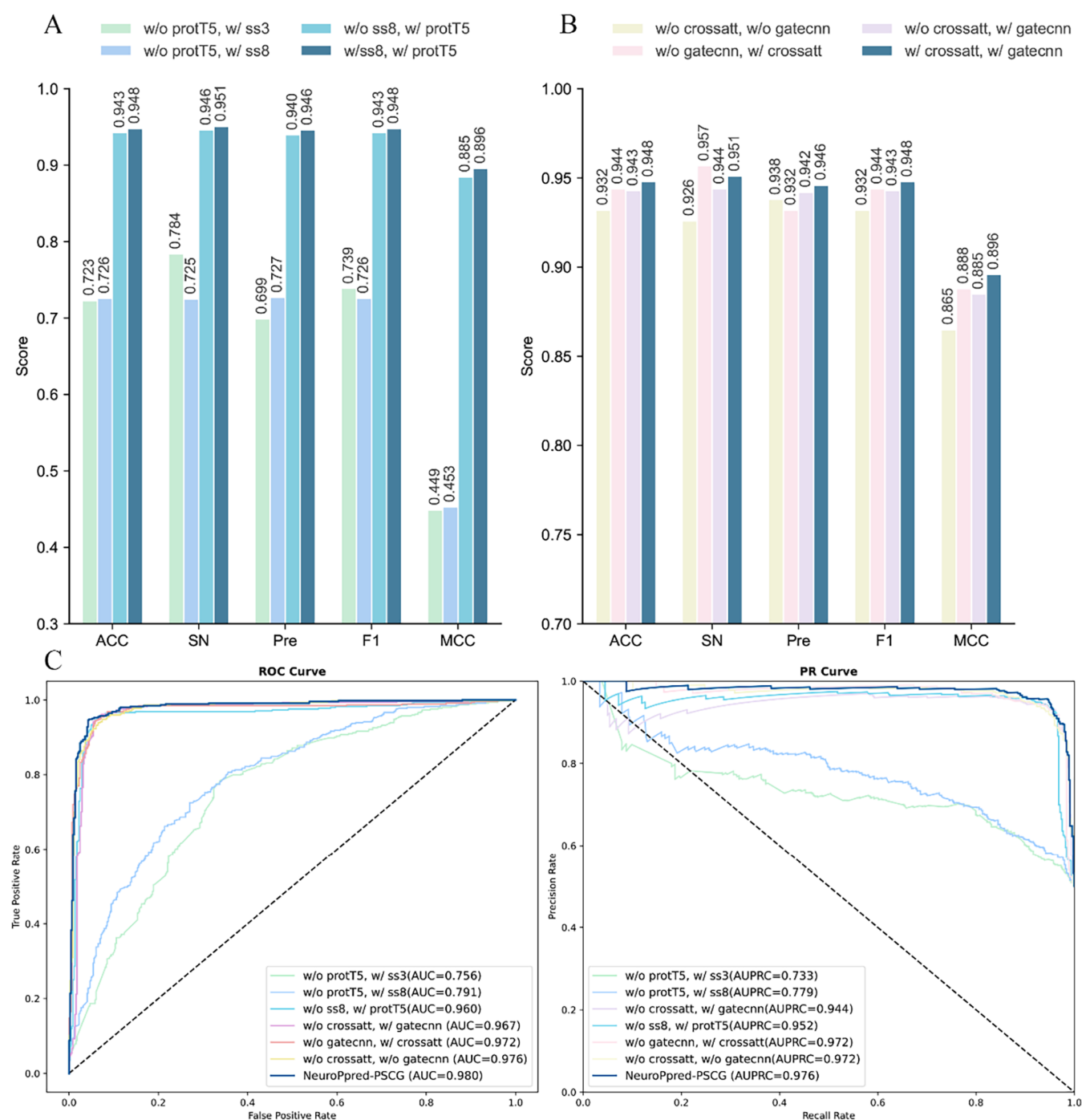
Figure 3. Results of the ablation study. (A) Effectiveness of multimodal features. (B) Contribution of cross-modal fusion mechanisms. (C) ROC and PR curves.
