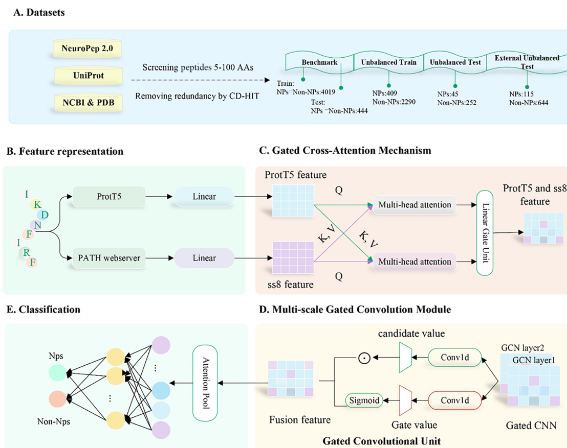
Figure 1. Flowchart of the NeuroPred-PCSG model. (A) Data set construction and preprocessing. (B) Feature representation based on ProtT5 embeddings and predicted secondary-structure features. (C) Gated cross-attention mechanism enabling bidirectional cross-modal interaction and adaptive fusion. (D) Multiscale gated convolution module for extracting hierarchical contextual features. (E) Classification module for neuropeptide identification.
