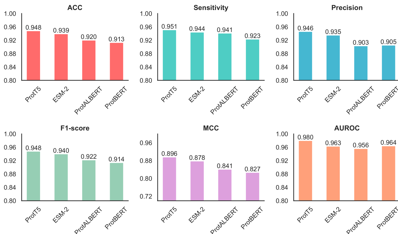
Figure 2. Performance comparison of different pretrained protein language models.
