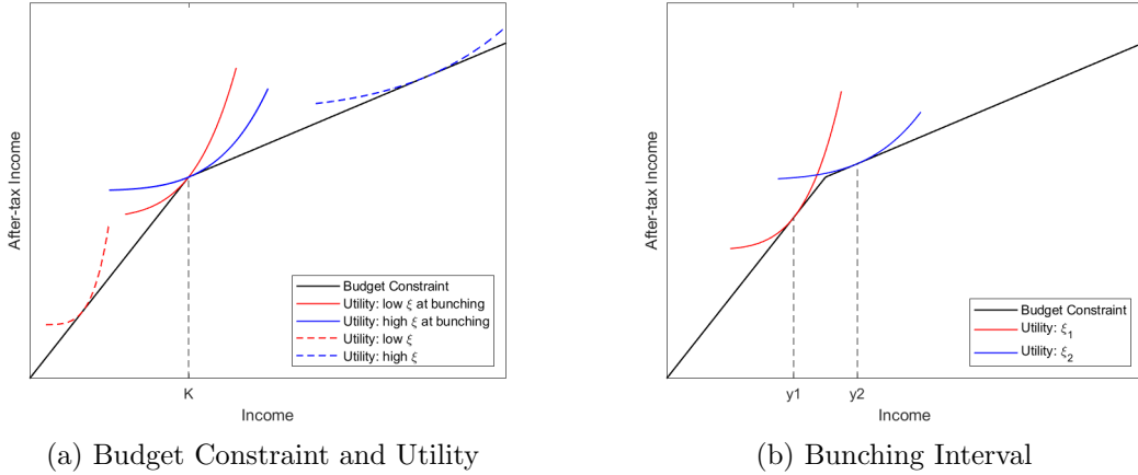
Figure 1: Example 2 Bunching and Taxable Income Elasticity
