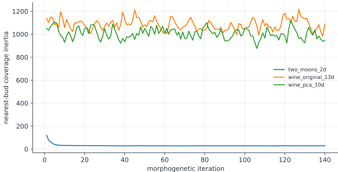
Finite-Step Bud Dynamics Before Compact Refinement
