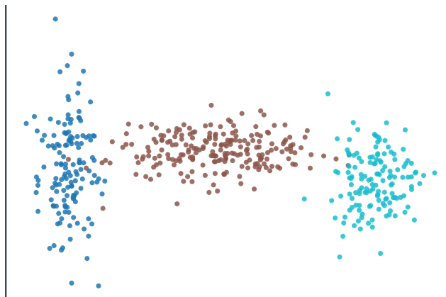
Varied Density
