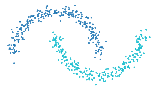
Two Moons
