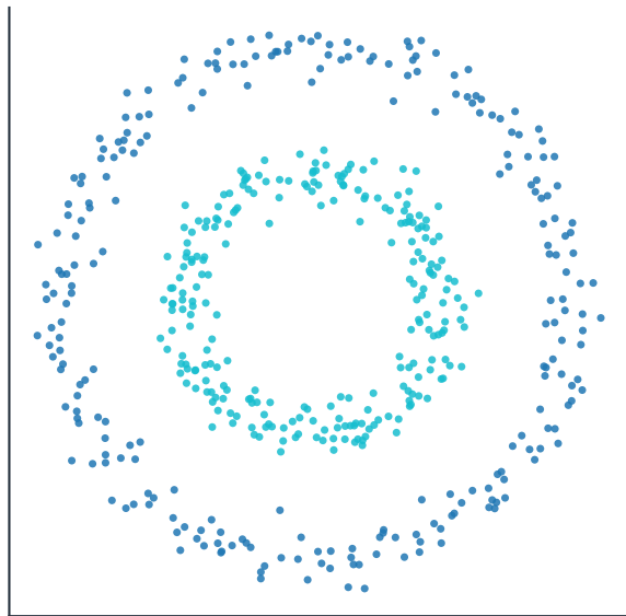
Noisy Circles
