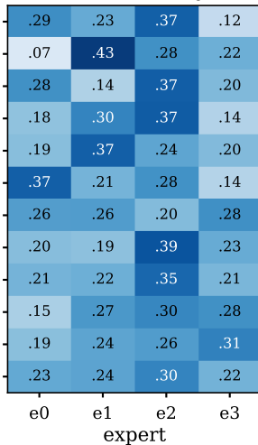
Shared + modality bias
