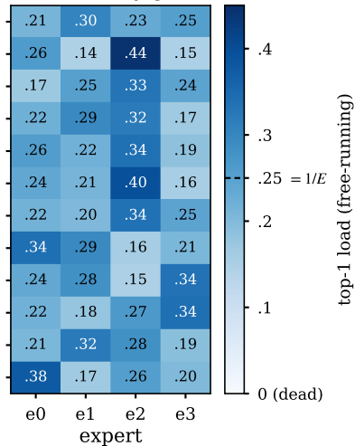
Per-modality gates
