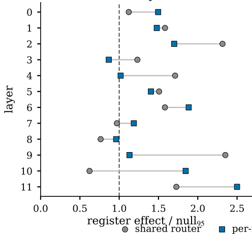
Melody stream 9/12 vs 10/12 layers above null
