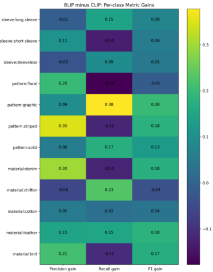
paper_per_class_metric_gains_blip_minus_clip.png
