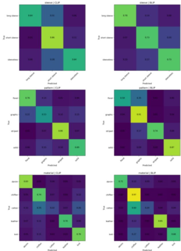
paper_normalized_confusion_matrices.png
