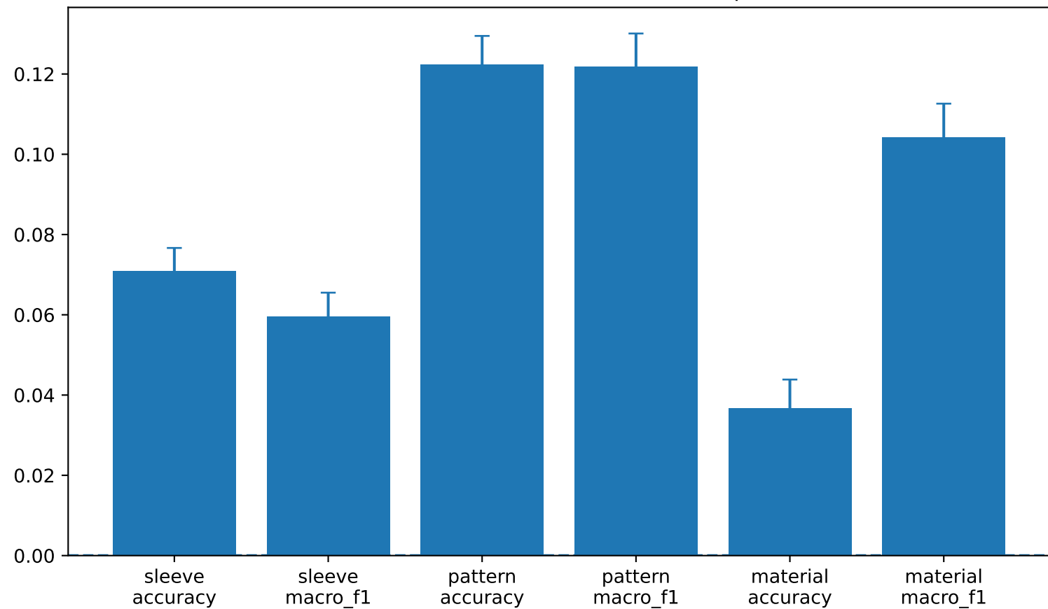
BLIP minus CLIP with 95% Bootstrap CI
