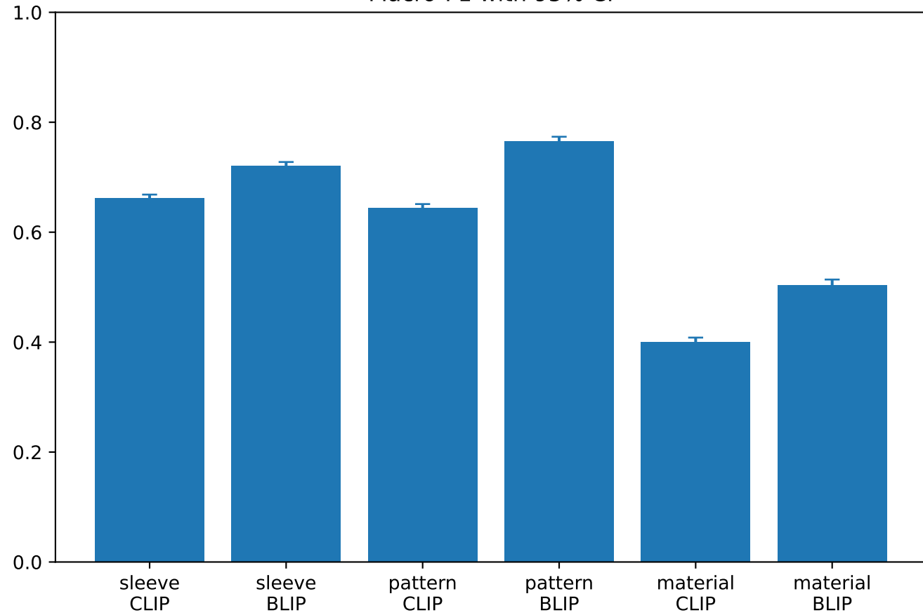
Macro-F1 with 95% CI
