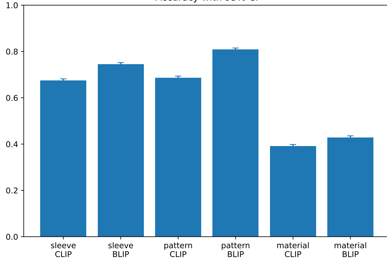
Accuracy with 95% CI
