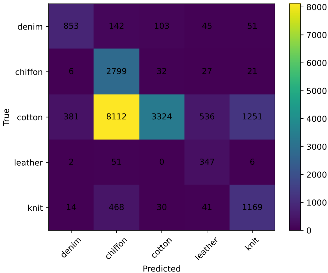
BLIP Confusion Matrix: material
