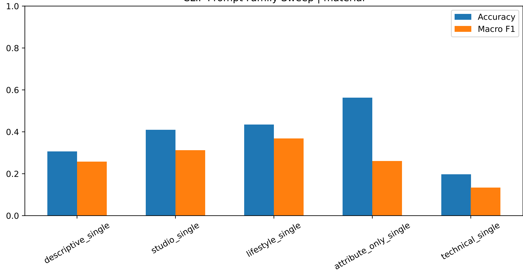
CLIP Prompt Family Sweep | material
