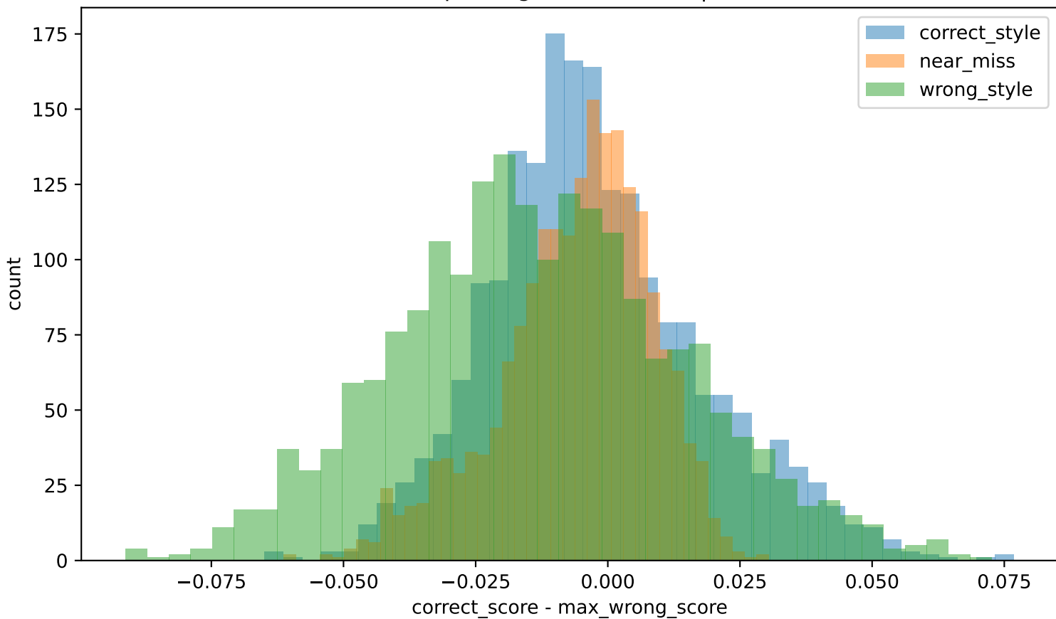
CLIP Prompt Margin Distribution | material
