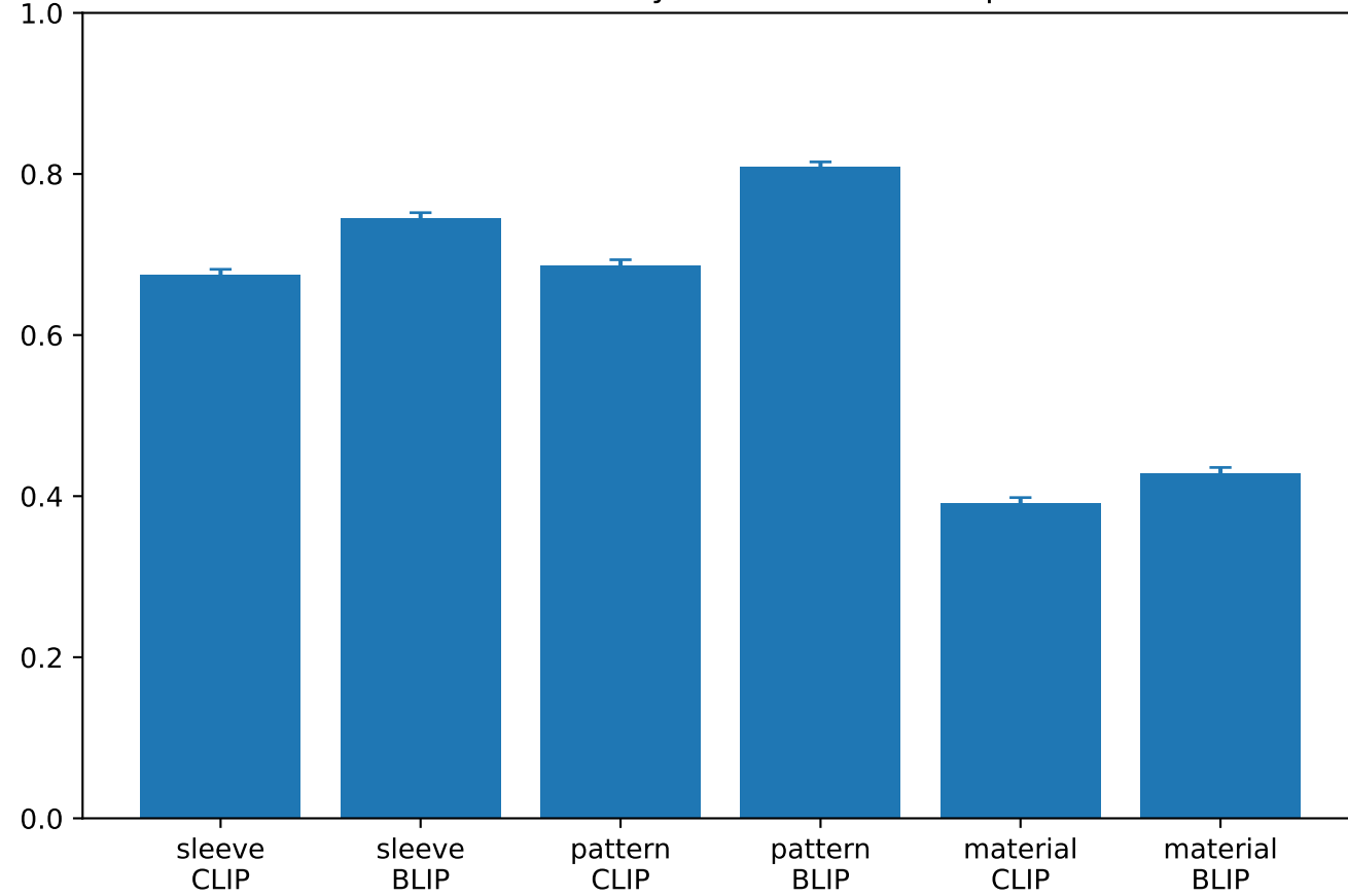
Overall Accuracy with 95% Bootstrap CI
