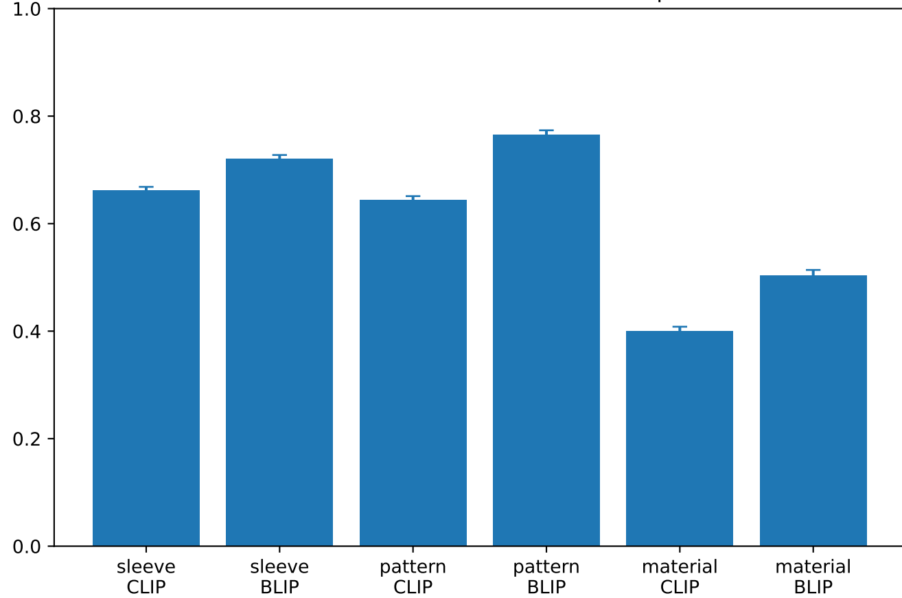
Overall Macro-F1 with 95% Bootstrap CI
