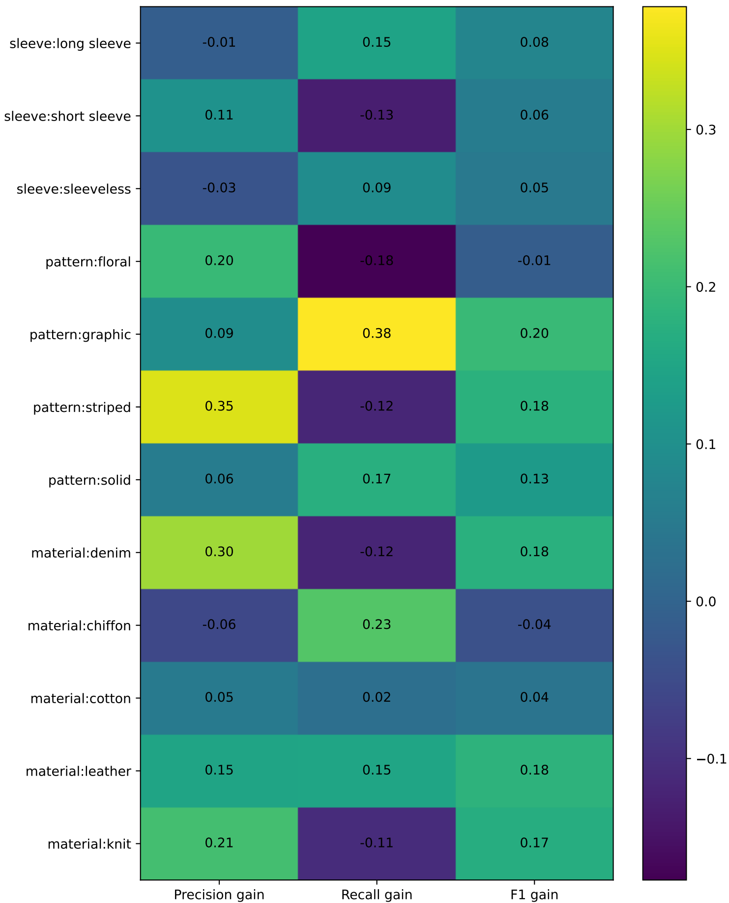
BLIP minus CLIP: Per-class Metric Gains
