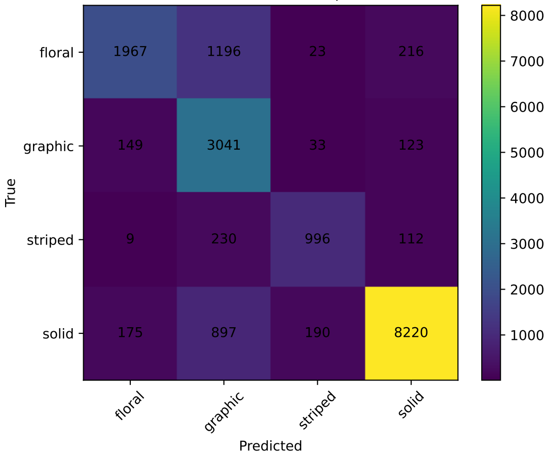
BLIP Confusion Matrix: pattern
