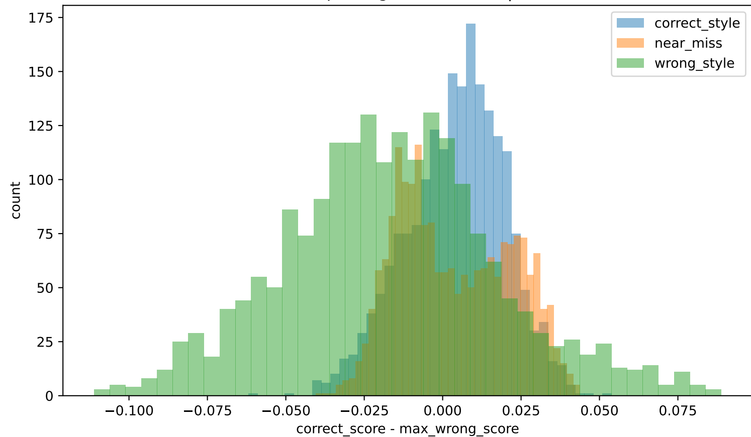
CLIP Prompt Margin Distribution | sleeve
