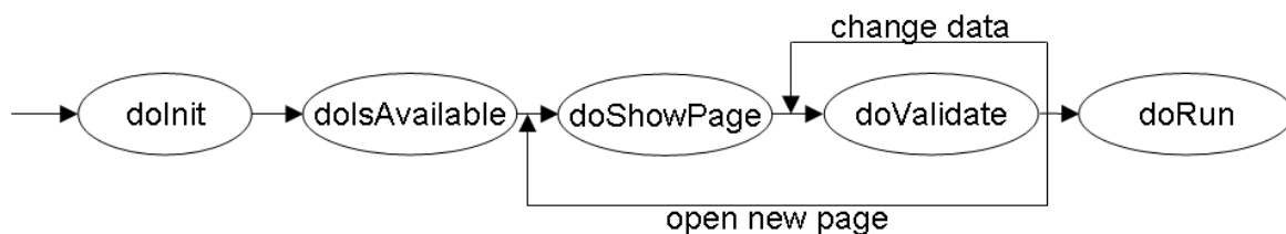
Figure 9.11. Wizard lifecycle
