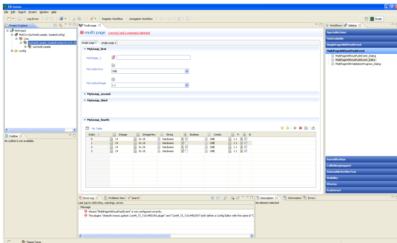
Figure 9.5. Standalone editor
