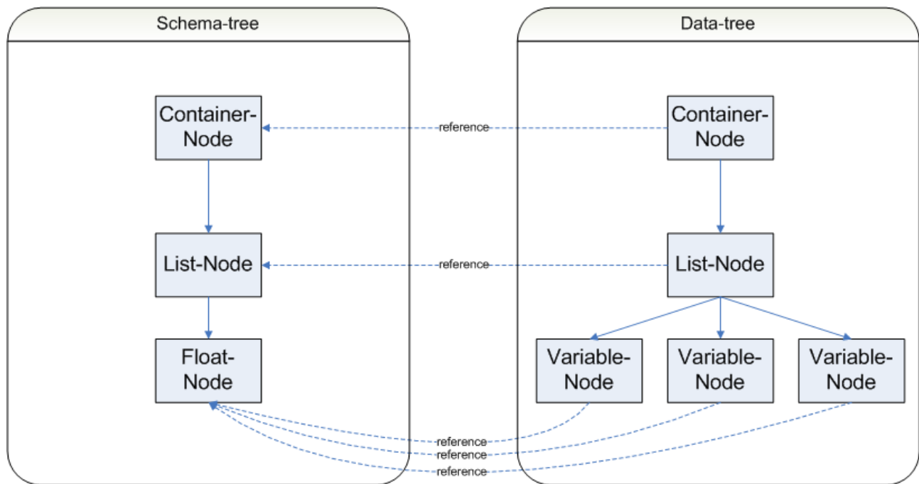
Figure 7.6. List-Representation
