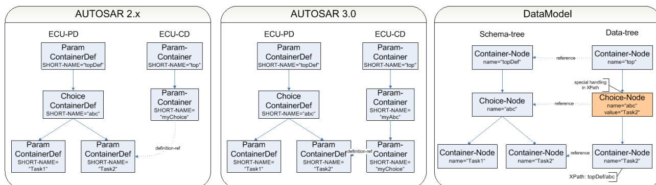
Figure 6.7. Choice-Representation
