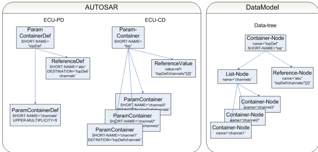
Figure 6.8. Reference-Example
