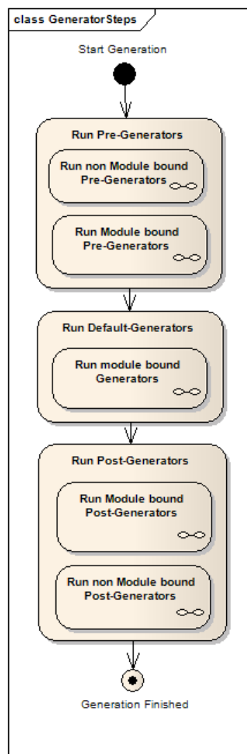
Figure 8.3. Generation Flow
