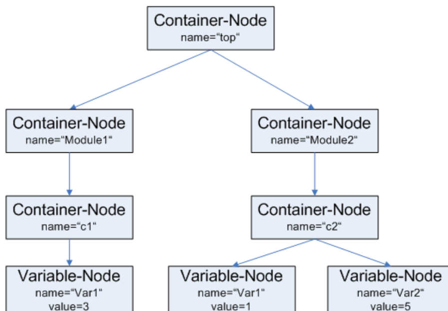
Figure 7.61. Example-Tree
