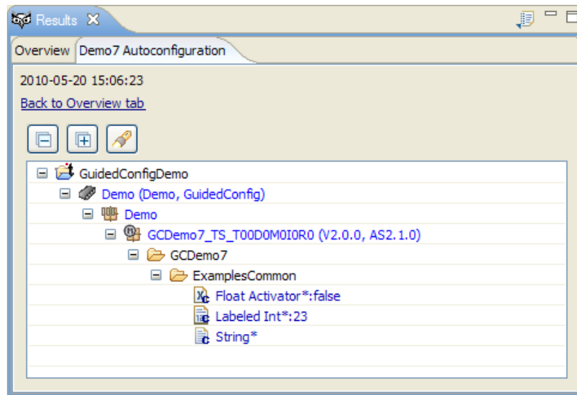
Figure 9.20. ChangedDCtxtsResultWidget
