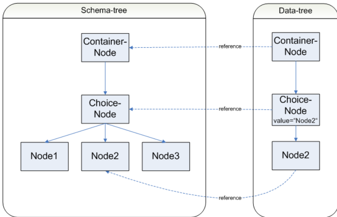
Figure 7.7. Choice-Representation
