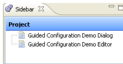
Figure 9.52. Sidebar view
