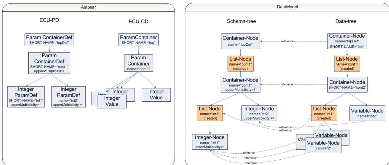
Figure 6.6. List-Representation
