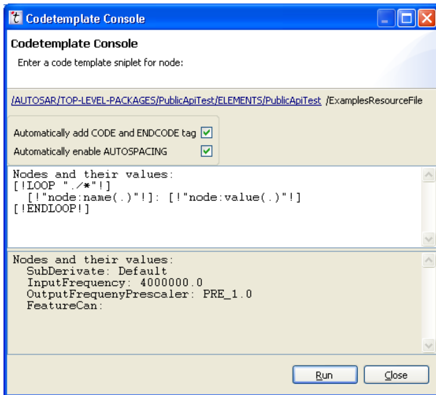
Figure 8.2. Codetemplate Console
