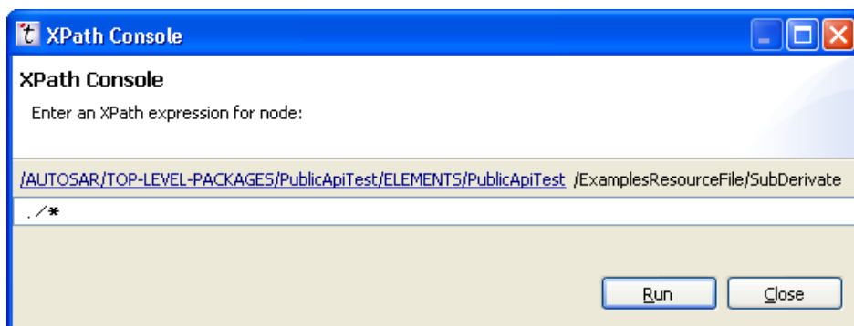
Figure 7.59. XPath Console
