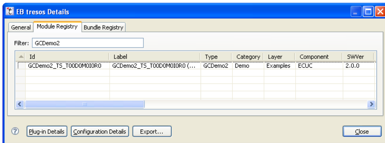
Figure 9.55. Module Registry
