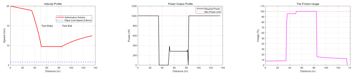
Figure 18: Comparison of Effects
