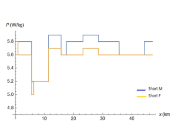
(a) P_{out}(x) plot for sprinters
