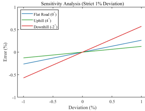
Figure 22: Slope Gradient Sensitivity Analysis
