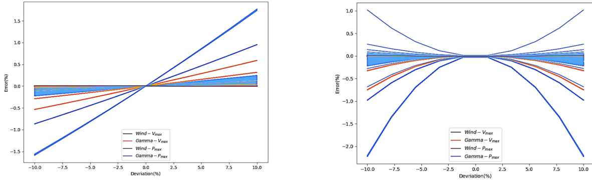
Figure 21: Sensitivity of wind speed&direction. Left: The course in Japan, with v_{wind} = 2 m/s, \gamma = -45^\circ . Right: The course in Belgium, with v_{wind} = 2 m/s, \gamma = 180^\circ .
