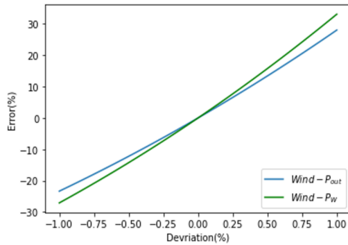
Figure 19: Sensitivity of wind speed
