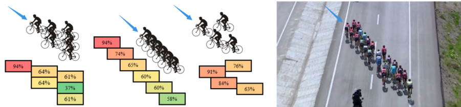
Figure 25: Left: Cycling strategy for lateral wind. Right: Slanted line array in Tour of Turkey 2016.
