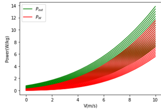
Figure 20: Change of P_{out}(v) and P_w(v)
