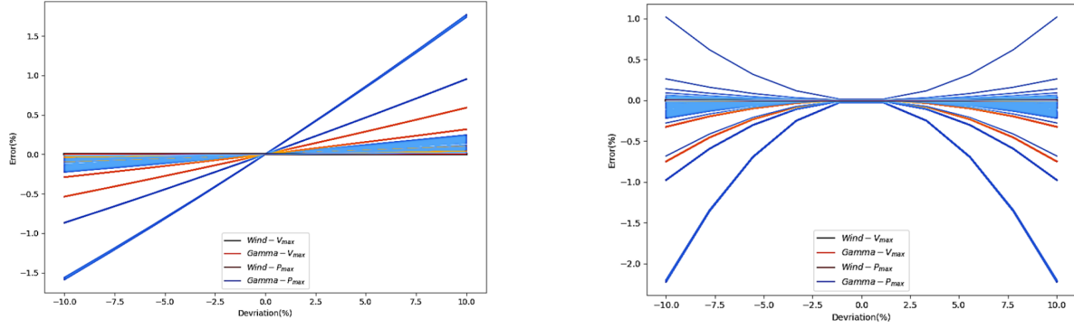
Figure 20: Sensitivity of wind speed&direction. Left: The course in Japan, with v_{\text{wind}} = 2 m/s, \gamma = -45^\circ . Right: The course in Belgium, with v_{\text{wind}} = 2 m/s, \gamma = 180^\circ .
