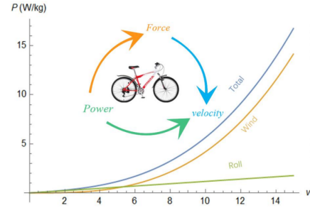
(b) P_{\text{out}} - v plot
