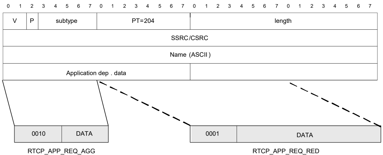
Figure 10.1: RTCP-APP formatting
