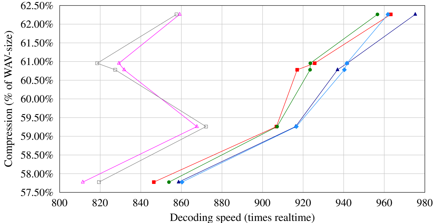
Decoding realtime speed vs compression for set of 16bit tracks vbuf SSD
