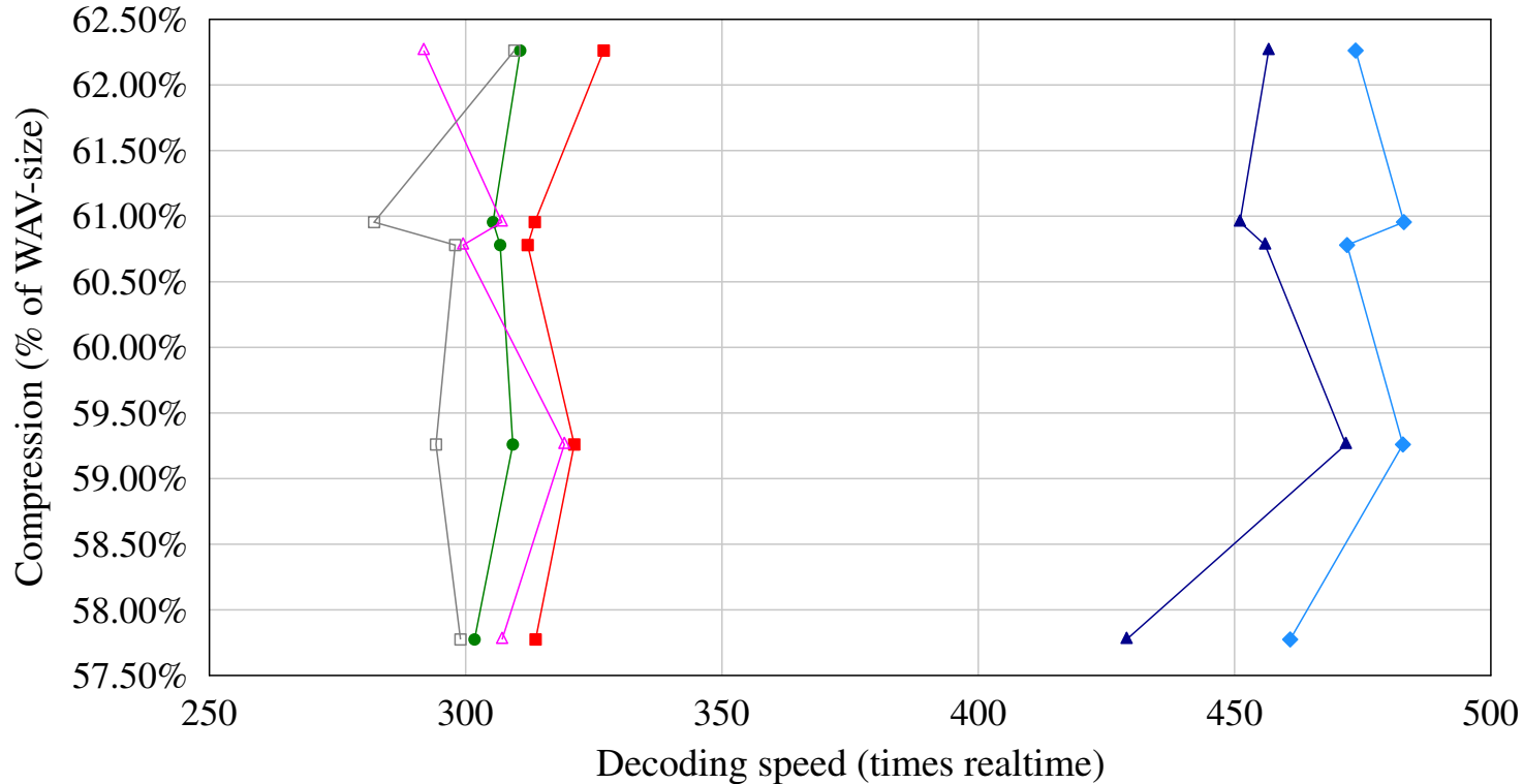
Decoding realtime speed vs compression for set of 16bit tracks vbuf HDD
