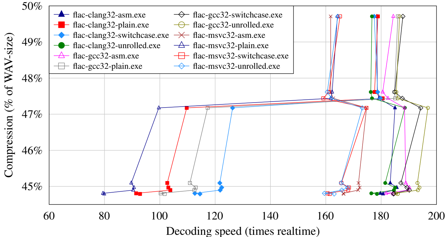
Decoding CPU speed vs compression for set of short tracks
