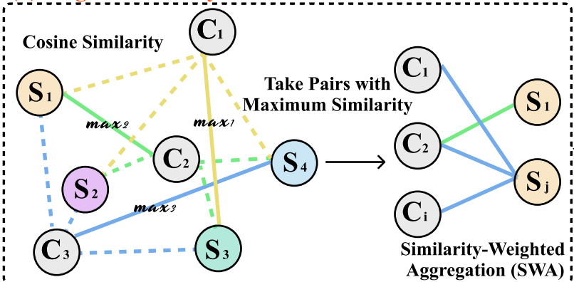
(d) Stage 3: Recovery from the Discarded via SWA
