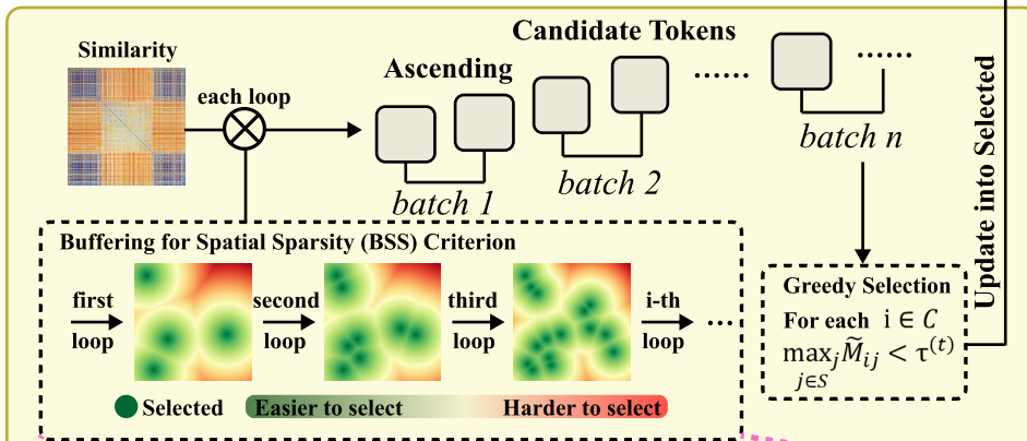
(c) Stage 2: Greedy Selection with BSS Criterion
