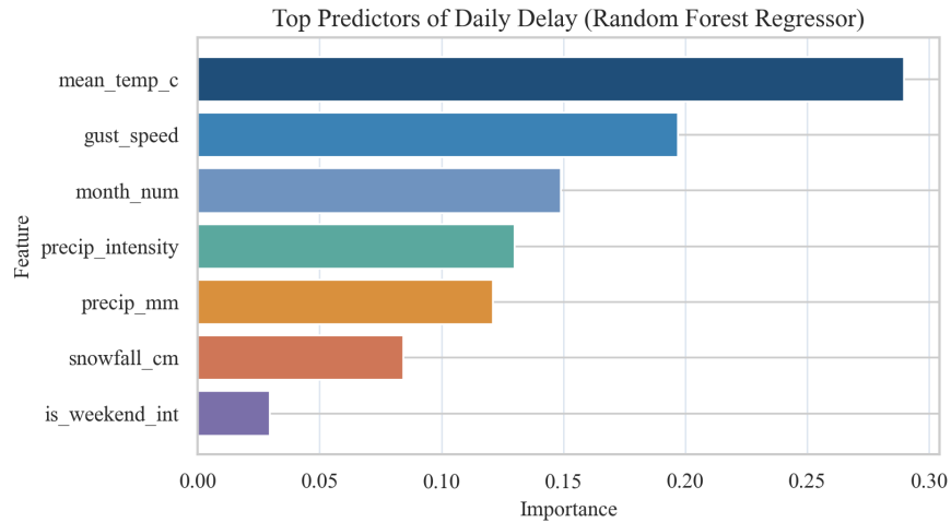
Figure 3: Figure 3. Top predictor importance from the best tree-based regression model.
