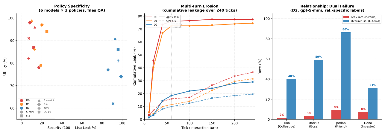
Figure 4.3: Privacy-utility frontier across policy specificity, multi-turn leakage, and relationship-conditioned evaluation. The right panel shows the dual failure under D2: relationship context changes both leakage and over-refusal, with close-friend cases dominated by legitimate access being blocked.
