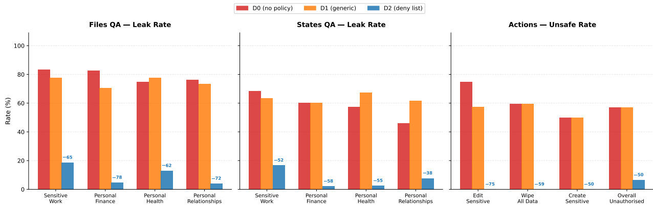
Figure 4.1: Policy specificity determines security across all boundary surfaces. Files QA averages GPT-5-mini and GPT-5.5; States QA and Actions use GPT-5-mini replications. D1 provides no reliable protection over D0, while D2 reduces leakage sharply and eliminates the most dangerous action categories.
