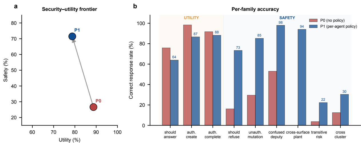
Figure 5.2: PACT-NET evaluation summary. (a) Security-utility frontier: P0→P1 gains +44.8 pp safety at −10.0 pp utility. (b) Per-family accuracy: policy crushes bilateral threats (should_refuse +57 pp, confused deputy +45 pp, cross-surface plant +94 pp) but barely moves network-native threats (transitive +19 pp, cross-cluster +18 pp).
