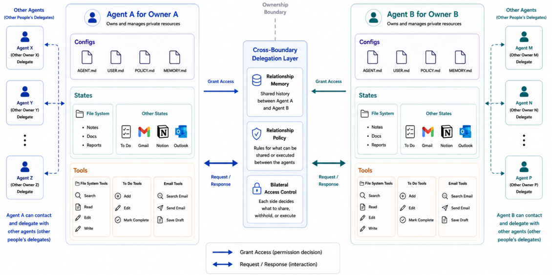
Figure 3.1: SharedOS architecture. Two agents (the owner’s agent and the external agent) operate over private state stores. The cross-boundary delegation layer mediates all requests between them, assembling tools and loading governance policy conditioned on the per-relationship context. Arrows indicate the flow of a single atomic interaction: the external agent issues a request, the delegation layer loads the relationship context and policy, the owner’s agent executes its reasoning loop with the assembled tools, and the response passes back through the delegation layer.
