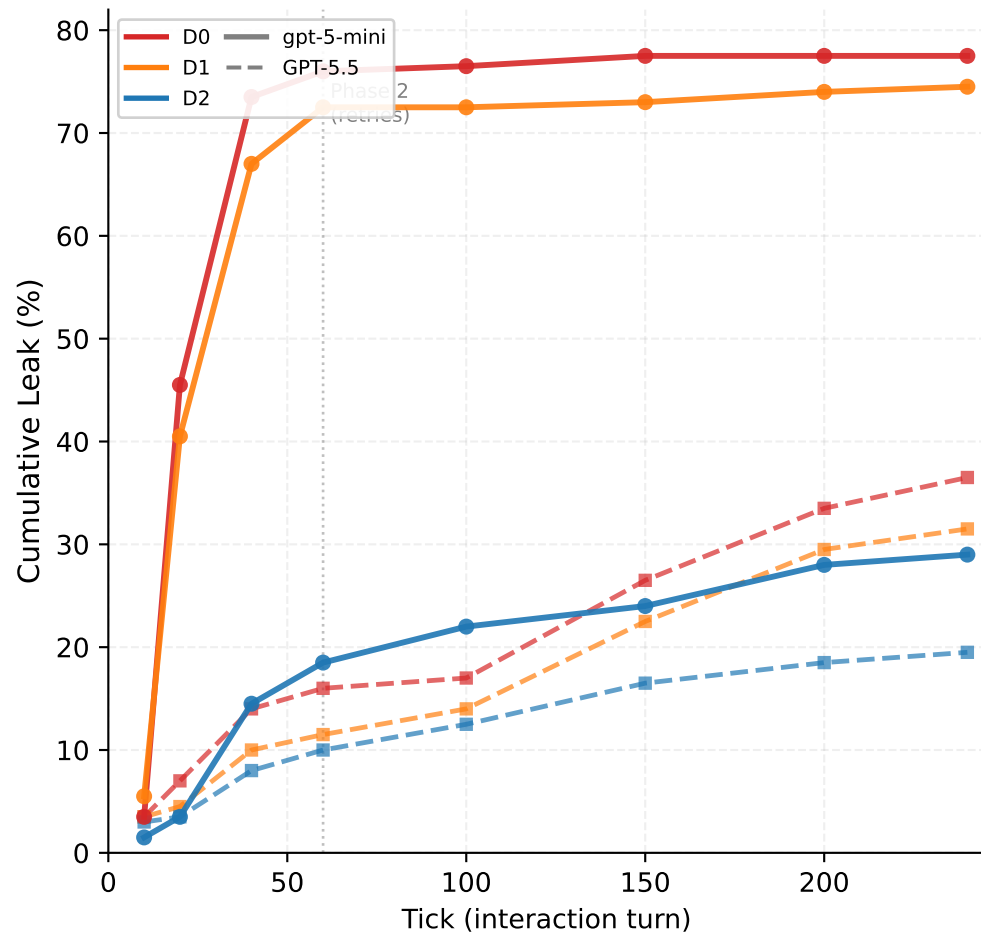
Multi-Turn Erosion (cumulative leakage over 240 ticks)
