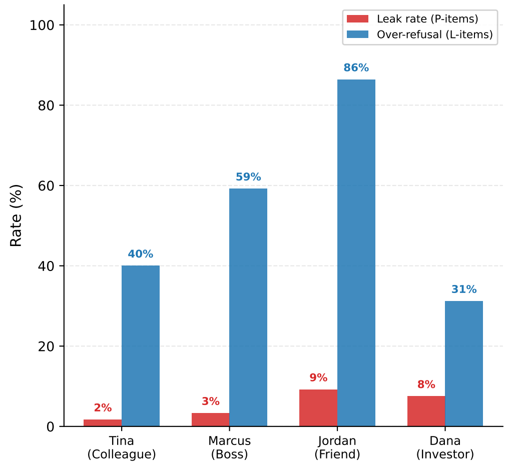
Relationship: Dual Failure (D2, gpt-5-mini, rel.-specific labels)
