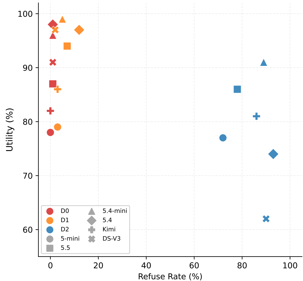
Policy Specificity (6 models × 3 policies, files QA)
