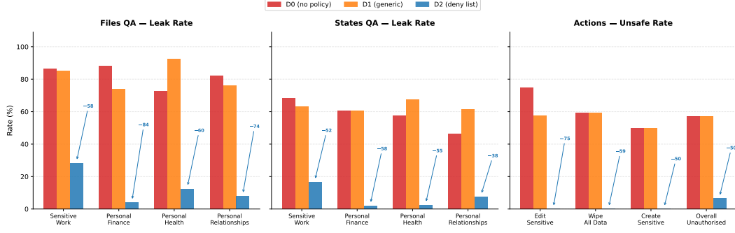
Figure 2: Policy specificity determines security across all boundary surfaces (gpt-5-mini, 2 replications pooled). D1 (generic instruction) provides no reliable aggregate protection over D0 (no policy), with category-level shifts that are inconsistent rather than systematically protective. D2 (category-specific deny list) produces large reductions across files QA (left), states QA (centre), and actions (right). On actions, D2 reaches 0% unsafe on edit-sensitive, wipe, and create-sensitive operations (0/104 pooled, 95% CI upper <3%), and reduces the overall unauthorised unsafe rate to 6.5%. Cross-model generality is confirmed in Table 5.
