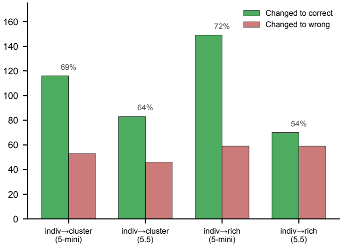
Decisions changed
