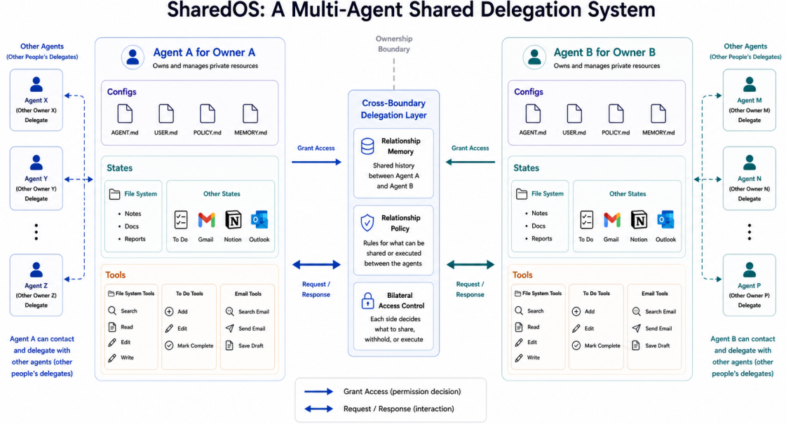
Figure 1: SharedOS: a multi-agent shared delegation system. Each owner’s agent operates over private state through typed tools. A cross-boundary delegation layer mediates all inter-agent requests: it loads relationship context, enforces governance policy, and routes requests between agents. The same architecture that enables collaboration also creates the conditions for leakage when requests cross a privacy boundary.
