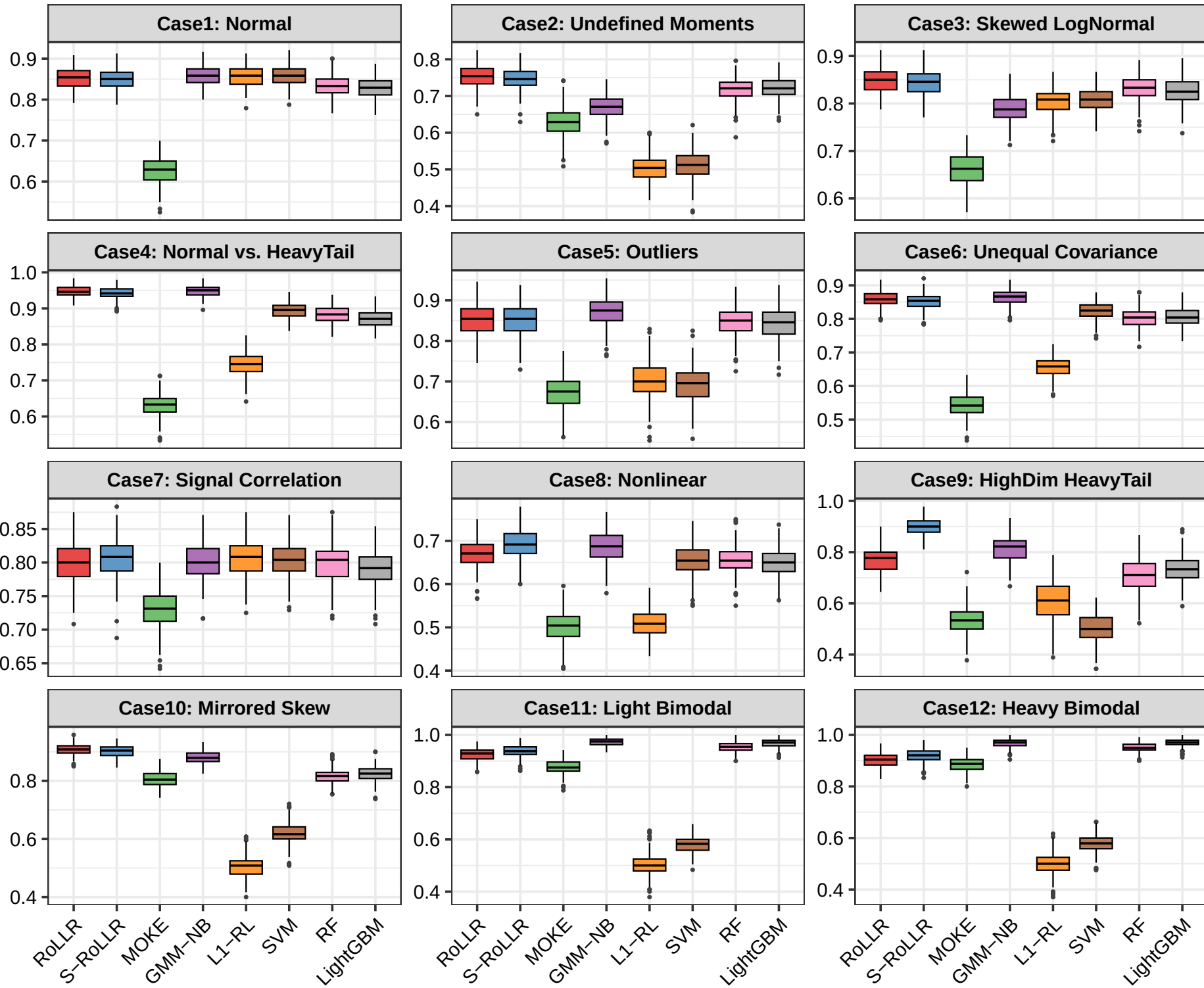
Accuracy
