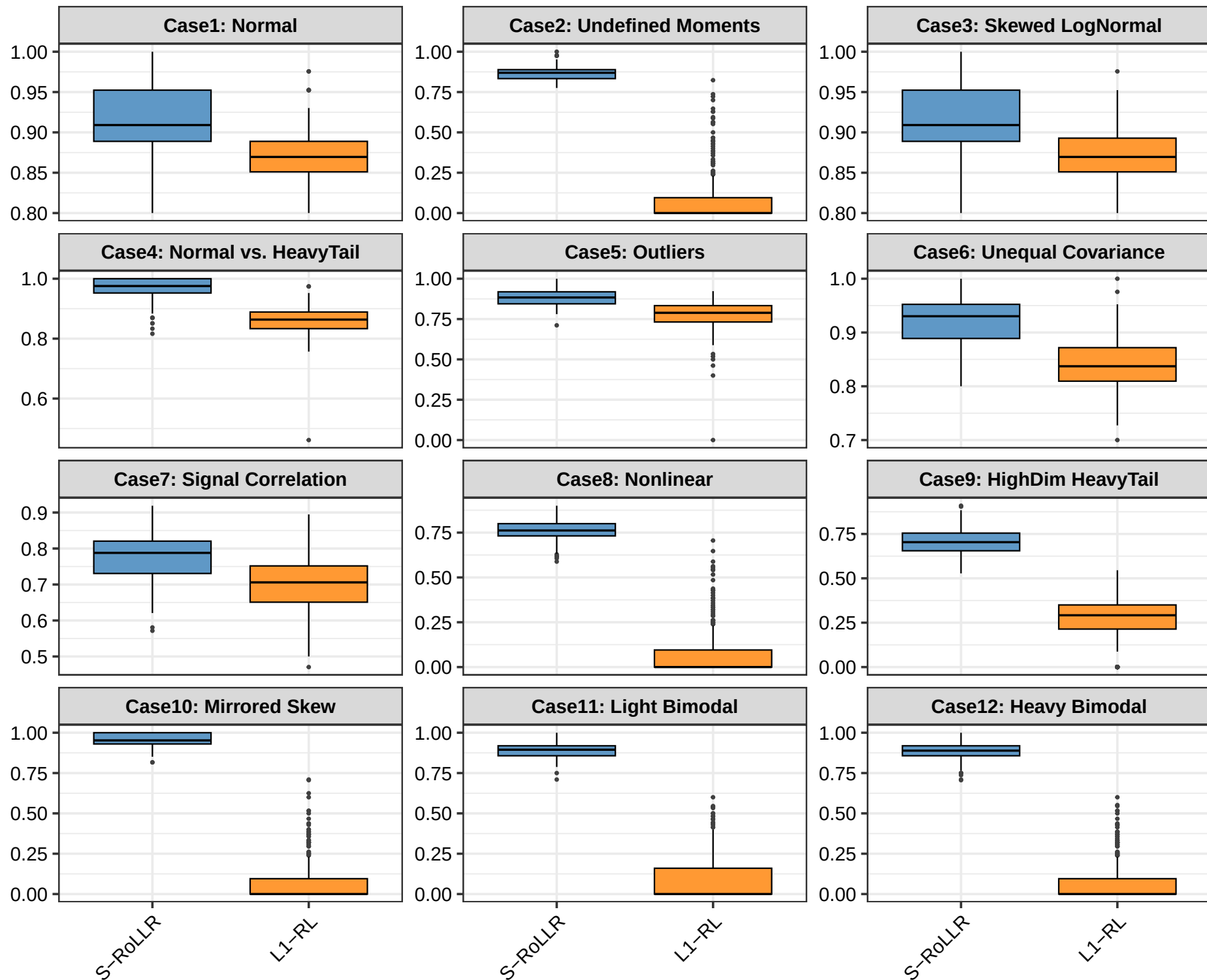
Selection F1-Score
