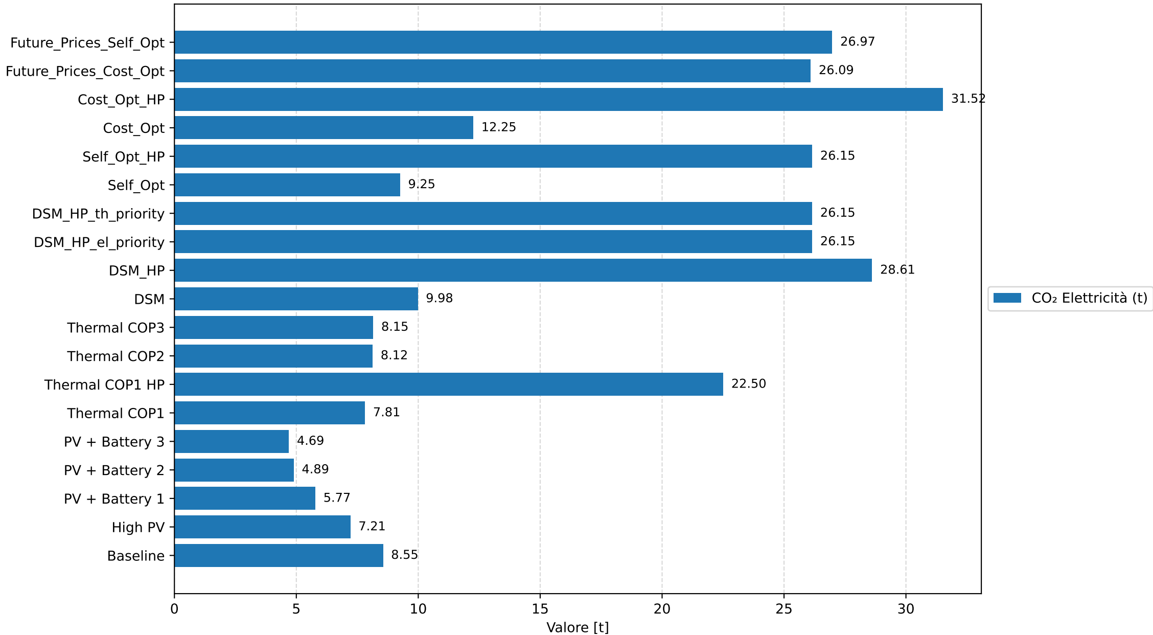
Emissioni (stack)
