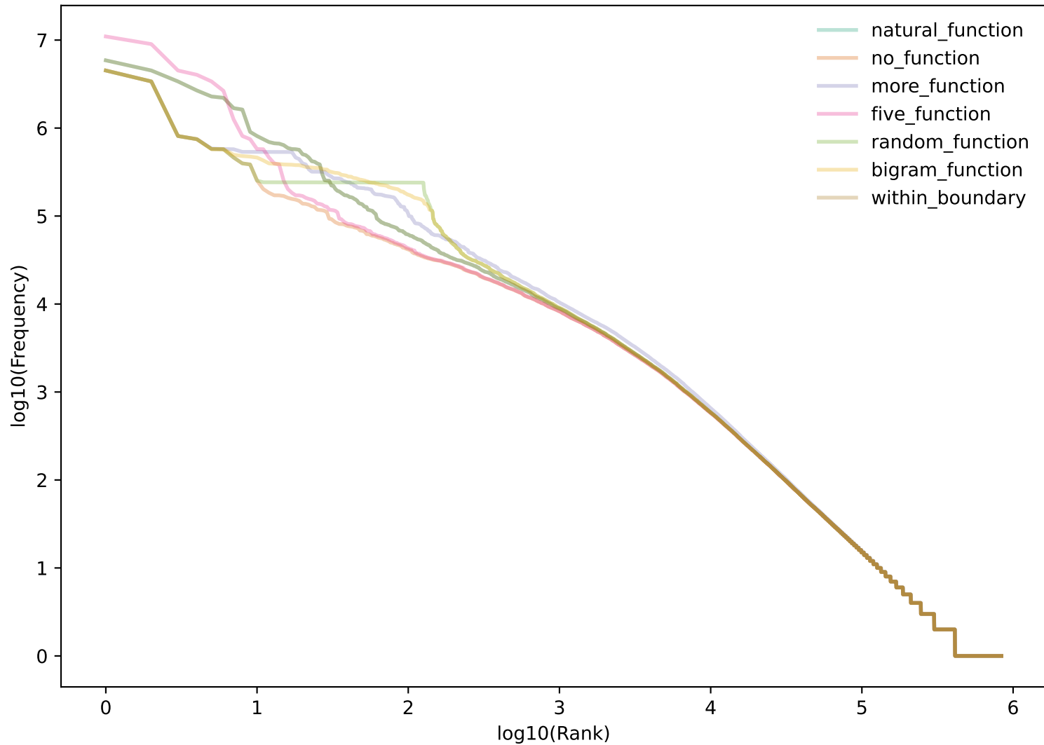
Zipf Distributions Across Function-Word Conditions
