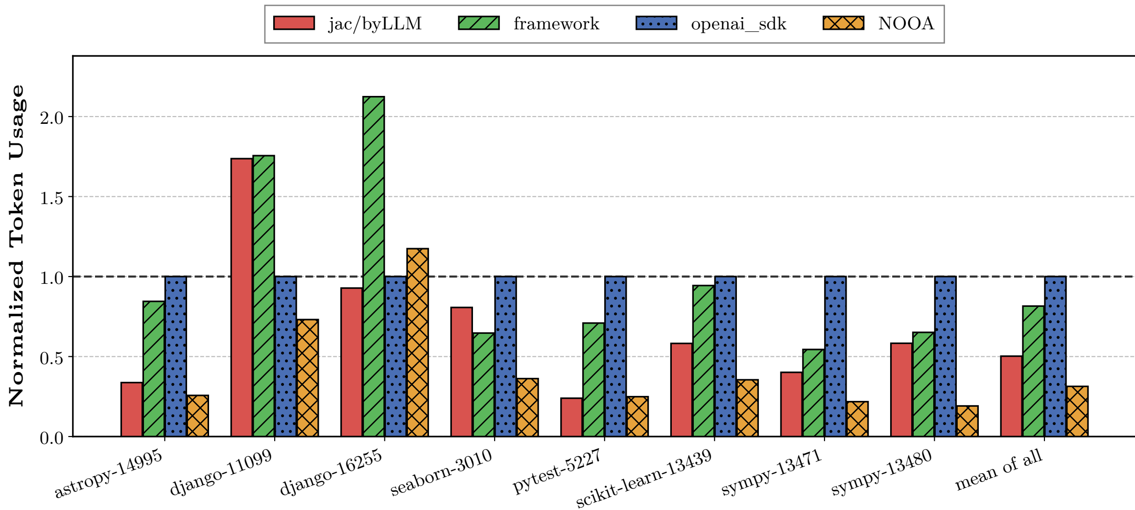
CodeAgent, SWE-bench Lite, 8 leaderboard-easy instances. Prompt + completion tokens per instance over openai_sdk's on the same instance. 1.0 = the openai_sdk baseline; lower is cheaper. Model: muse-glimmer (30B) via local ollama.
