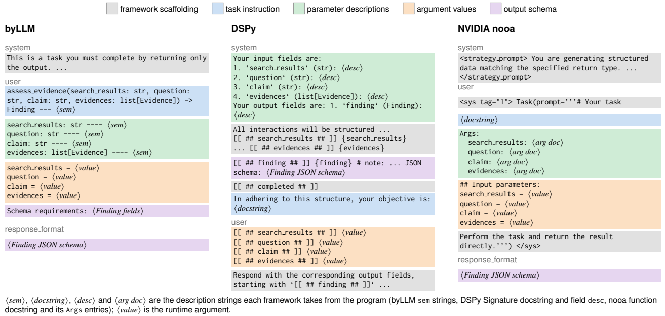
Figure 2. The prompt structure of LLM invocation function assess_evidence , lowered by three frameworks. They have similar structures: Same five kinds of component, only relative position differs.
