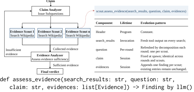
Figure 1. Heterogeneity within a HoVer-style [9] Fact Check Agent’s generated prompt for the summary-making function. assess_evidence(search_results, question, claim, evidences) evaluates the sub-question against the accumulated evidence and search results, then answers it.
