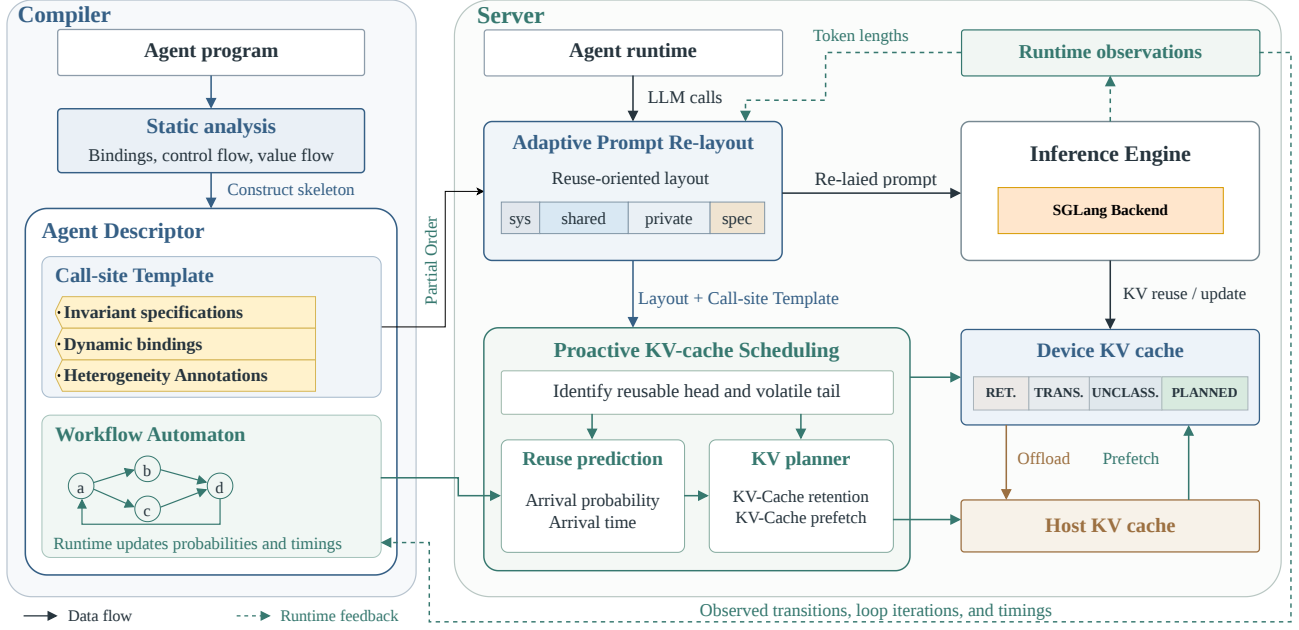
Figure 3. Architure overview of IDONTKNOWITSNAME.
