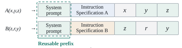
(b) Reordered layout
