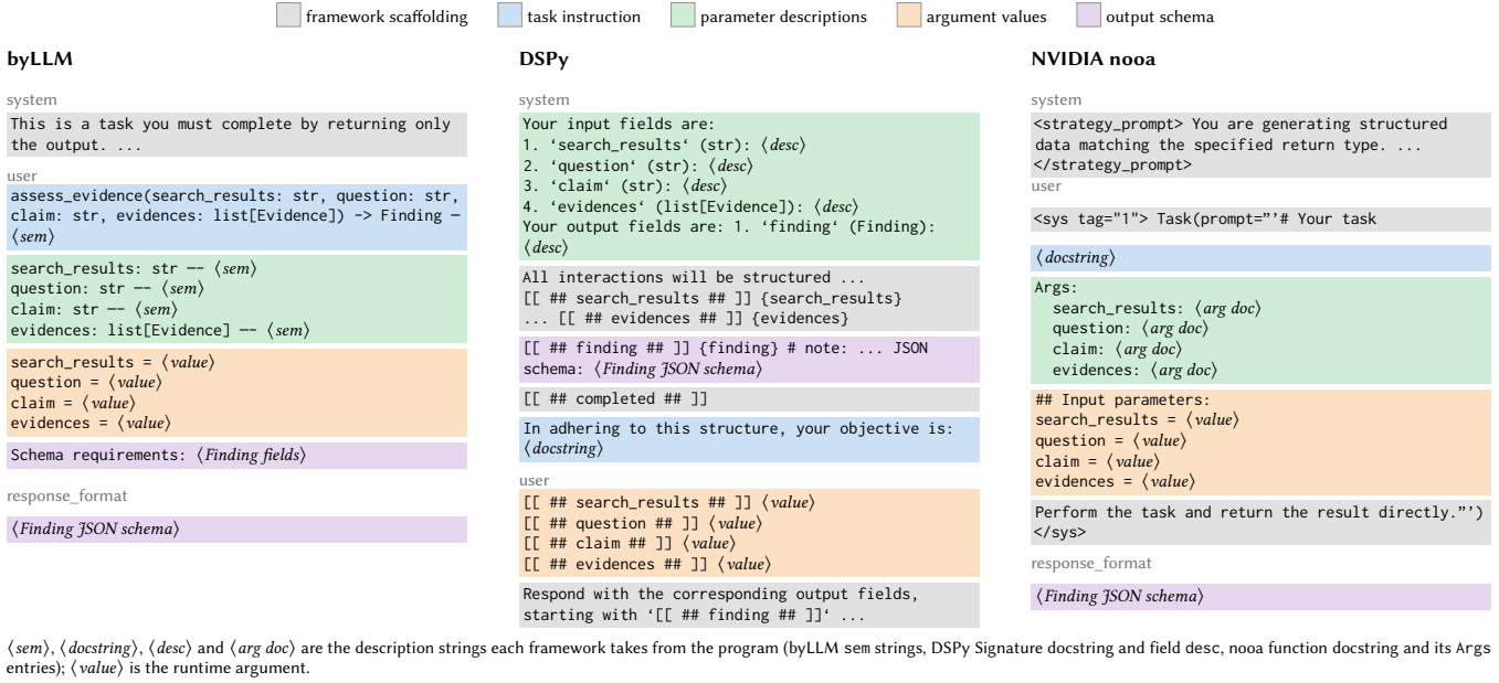
Figure 2. The prompt structure of LLM invocation function assess_evidence , lowered by three frameworks. They have similar structures: Same five kinds of component, only relative position differs.
