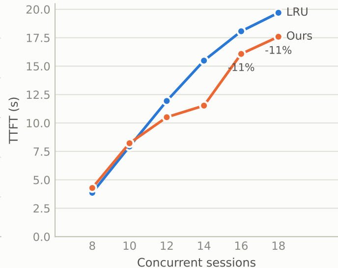
p95 TTFT, all calls
