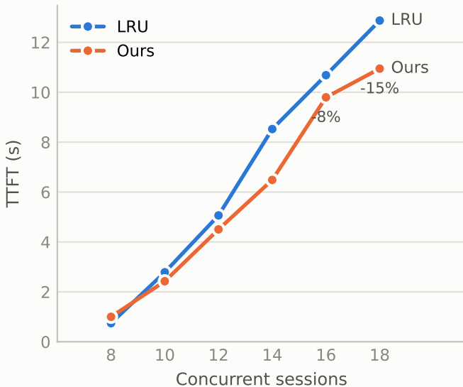
Median TTFT, all calls
