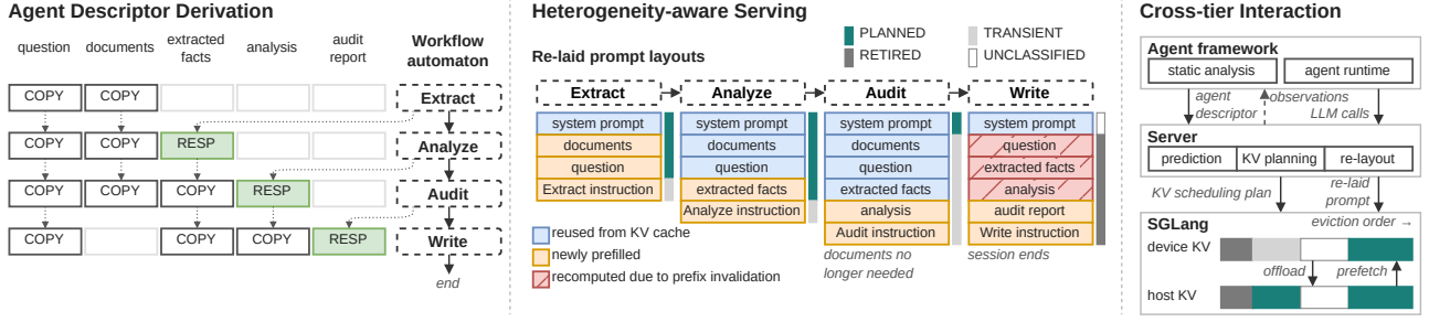
Figure 3. Architecture overview of ANON. Static analysis derives the agent descriptor, marking intra-prompt heterogeneity. The server uses it for KV-cache scheduling.
