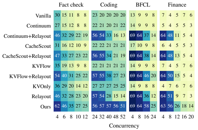
Figure 5. Cache hit rate (%) of prompt tokens under varying numbers of concurrent workflows.
