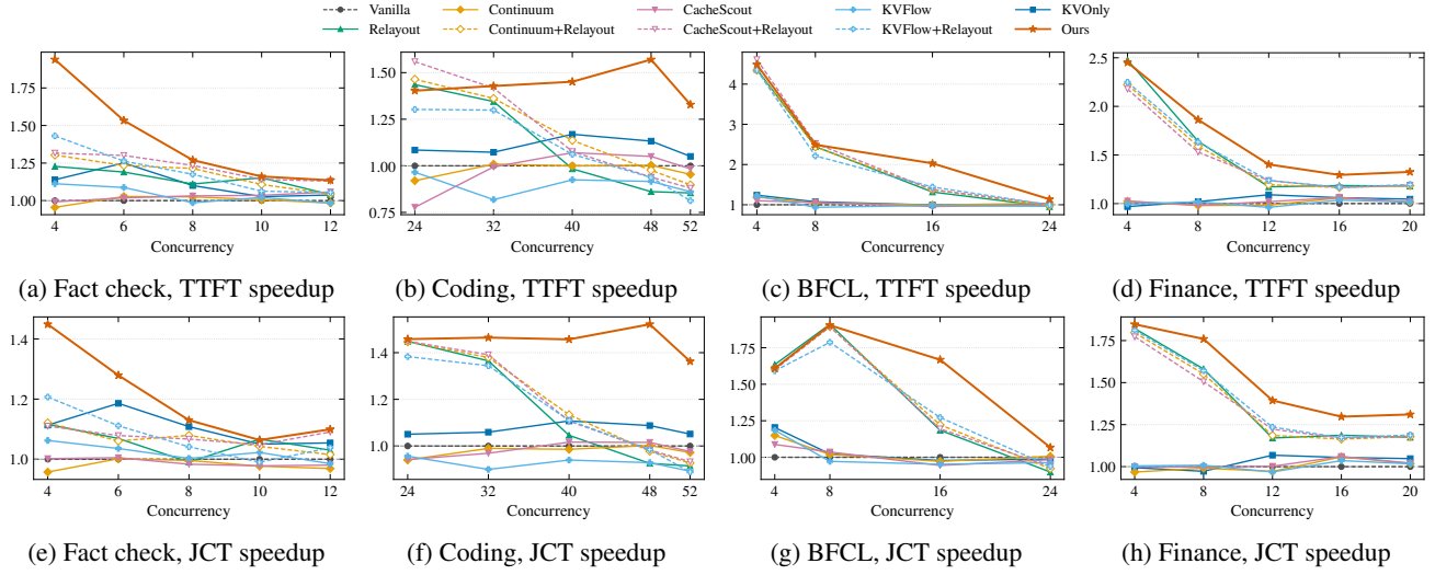
Figure 4. Average TTFT speedup (top) and average JCT speedup (bottom) over Vanilla SGLang under varying numbers of concurrent workflows.
