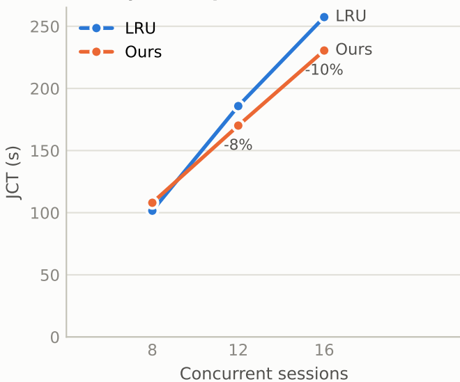
Mean job completion time
