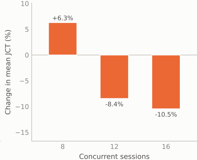
Ours relative to LRU, lower is better
