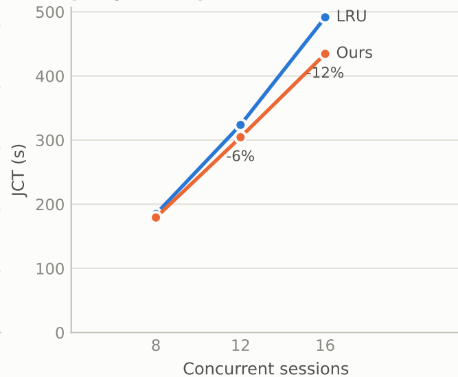
p95 job completion time
