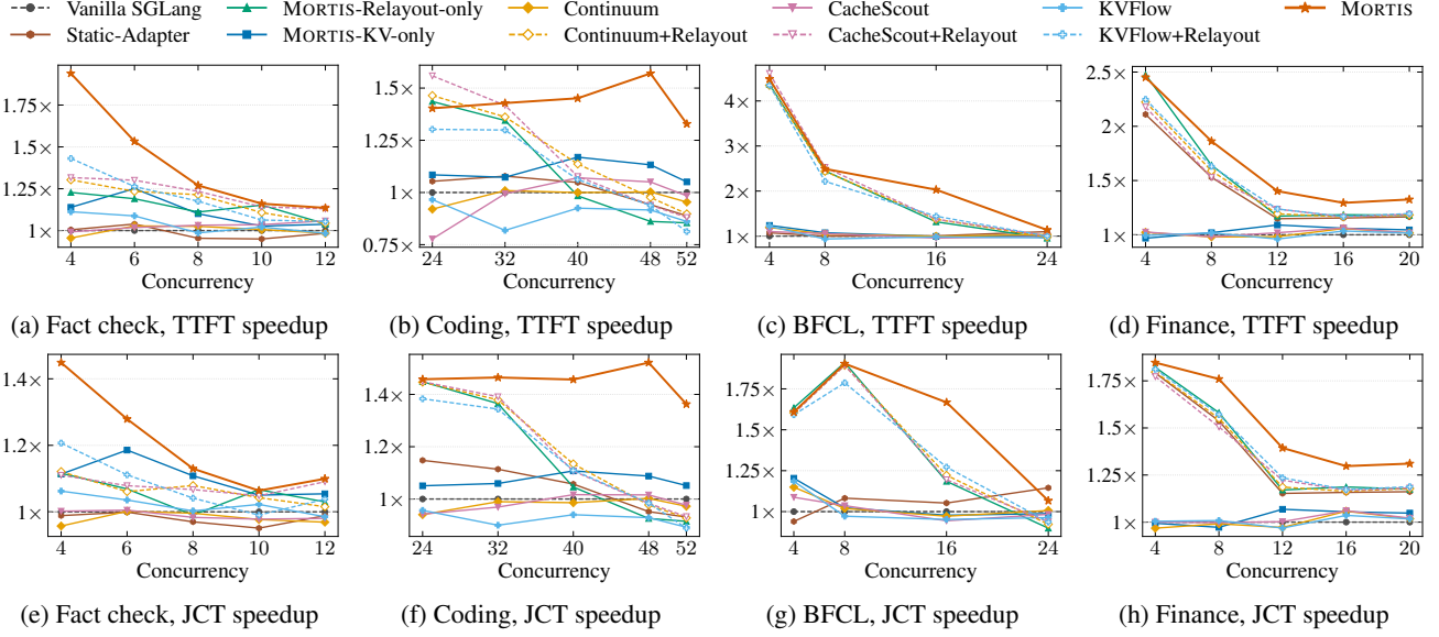
Figure 5. Average TTFT speedup (top) and average JCT speedup (bottom) over Vanilla SGLang under varying numbers of concurrent workflows.
