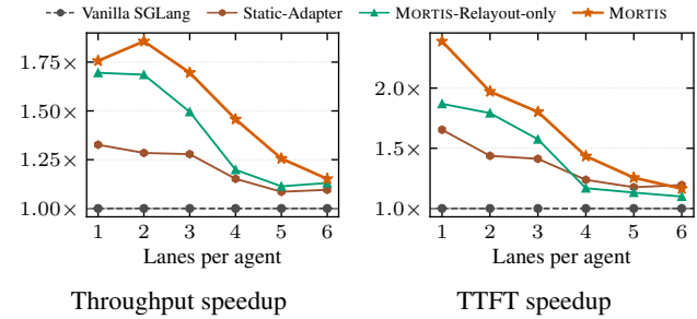
Figure 4. Throughput and average TTFT speedup over Vanilla SGLang under varying load on the mixed workload.
