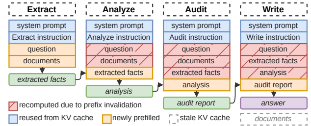
Figure 1. KV-cache reuse demonstration in a four-stage financial-analysis agent. This agent answers the question using the given documents. The stage-specific task instructions block KV-cache reuse, and the serving engine cannot proactively release the stale KV-cache ( documents after Audit here) without knowing the intra-prompt heterogeneity.
