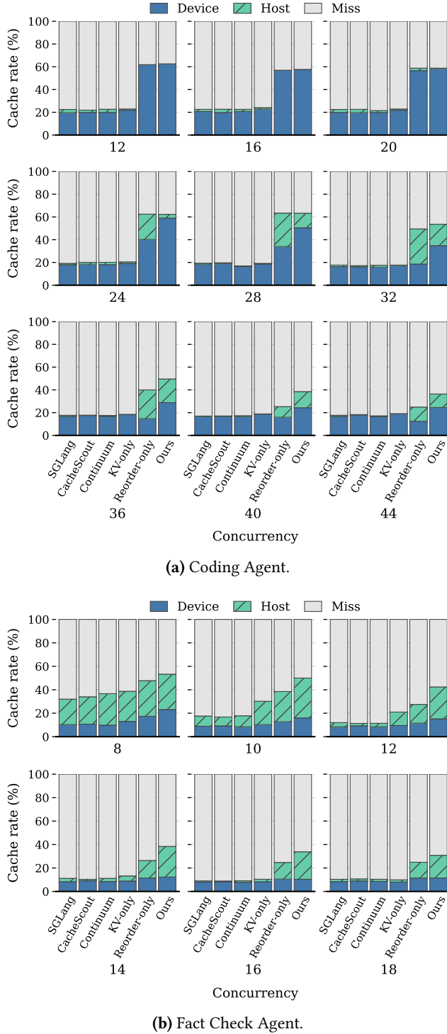
Figure 6. End-to-end KV-cache status (device hit, host hit, miss) under different concurrency levels.
